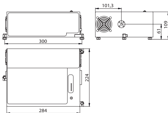
QX500 laser head outline drawing.
