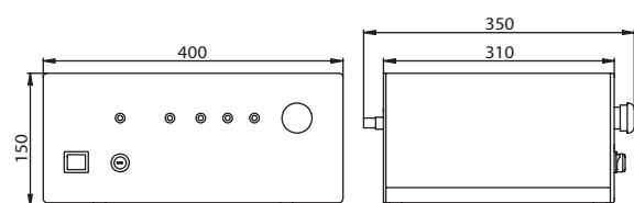
QX500 laser power supply outline drawing.
