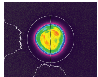
QX500 laser typical near field beam profile at 1064 nm.
